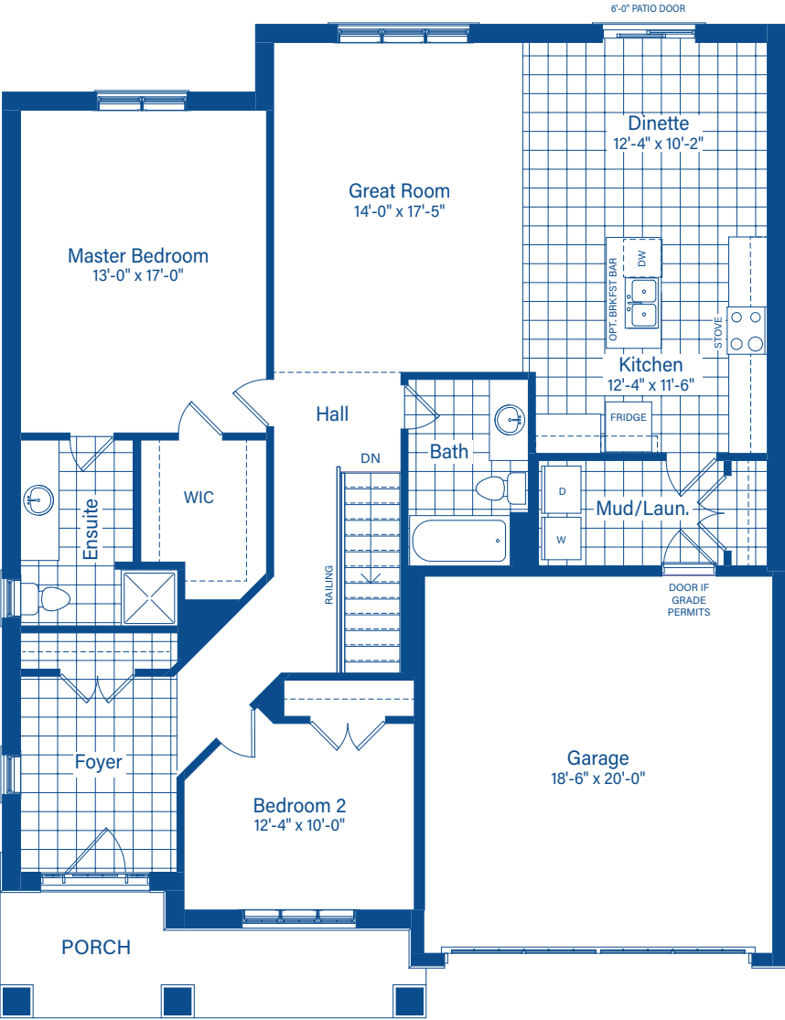
MAIN FLOOR
